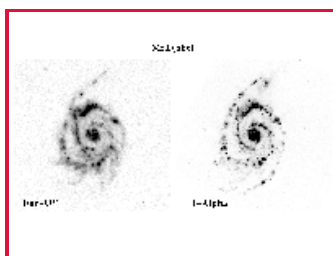
M51 (Spiral; Far-UV, H-alpha)
