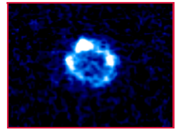
NGC 1317 (Sa Galaxy With Nuclear Ring)
