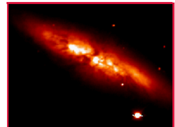
M82 (Starburst Galaxy With Galactic Wind)
