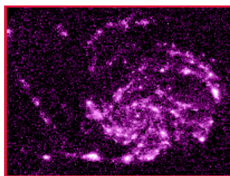
M74 (Spiral; Mid-UV, Optical)
