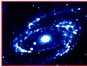
M81 (Spiral; Mid-UV, Optical)
