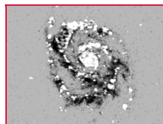
M51 (Far-UV, H-alpha Color Map)
