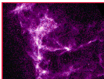
Cygnus Loop (Supernova Remnant)
