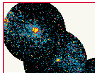
Small Magellanic Cloud Mosaic
