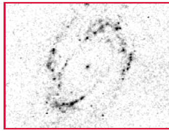
M81 (Far-UV, Mid-UV, Optical)
