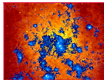
M33 UV/Optical Superposition
