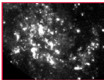
M33 (Spiral; UV/Optical Comparison, 4 Bands)
