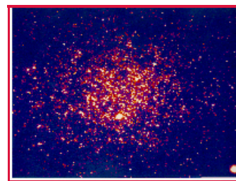
Omega Centauri (Center)
