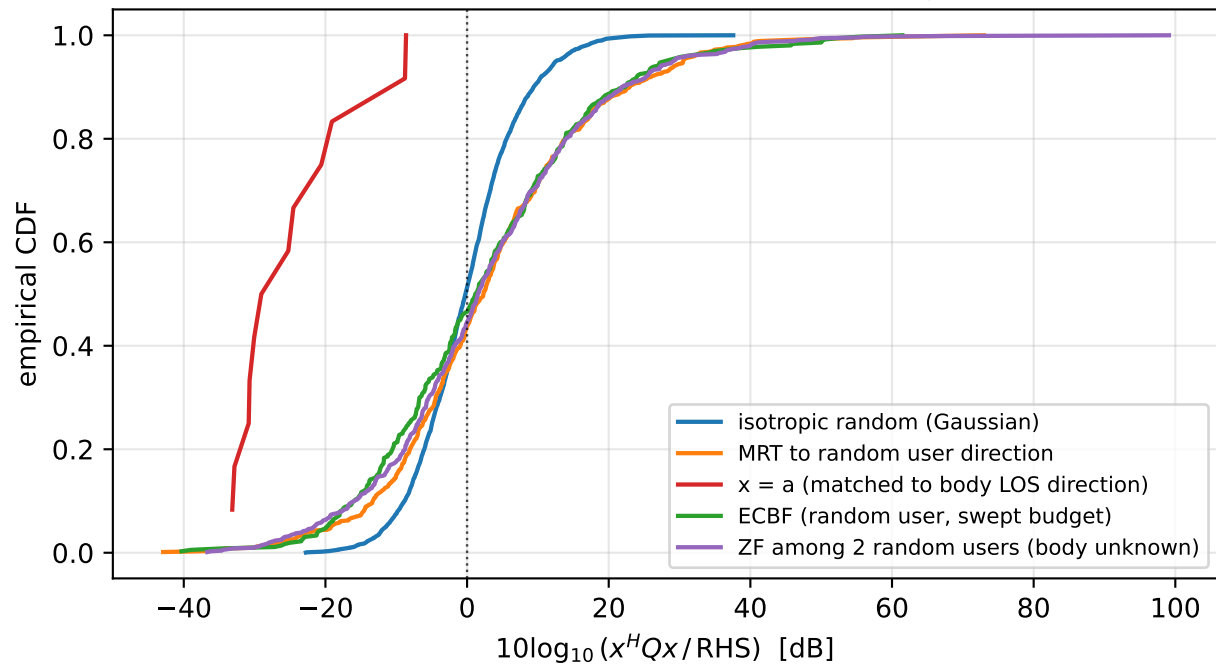
(b) 3GPP UMa-LOS (12 clusters x 5 subpaths)
