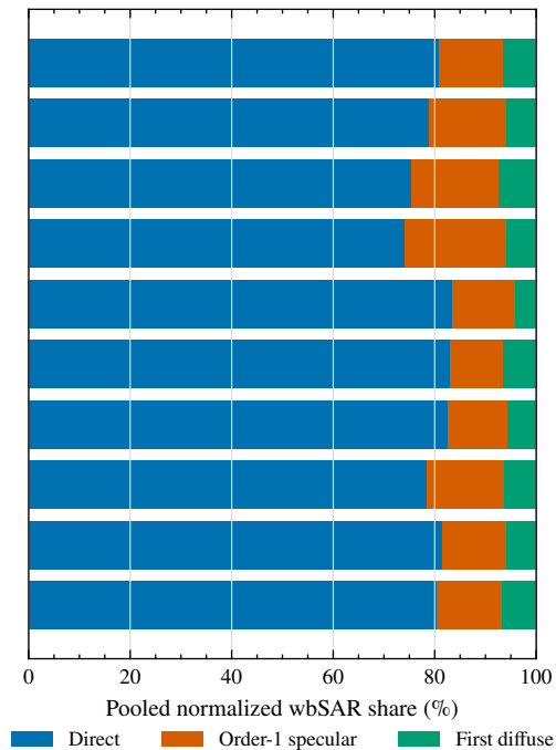
(b) First-interaction components
