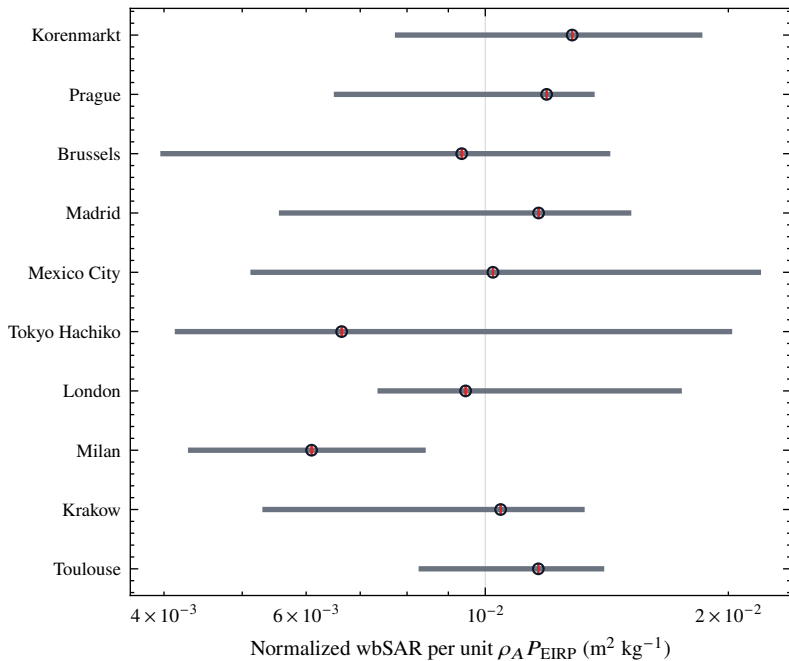
(a) Fixed-point q_{10} , q_{50} , and q_{90}
