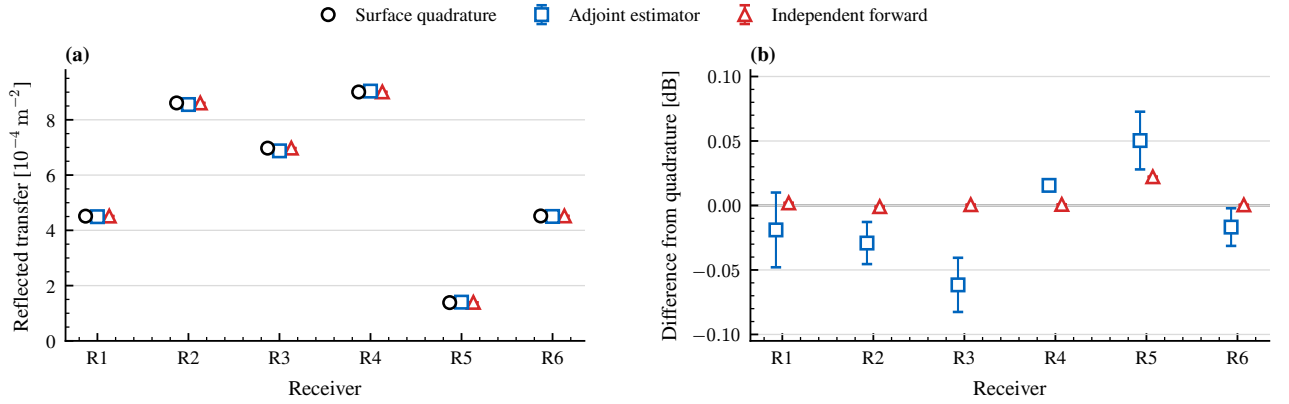
FIGURE 4. Controlled validation of the first-diffuse transfer. (a) Deterministic surface quadrature, the adjoint estimate, and the independent Sionna RT forward calculation at six receivers. (b) Signed error relative to quadrature. Error bars give the standard error across four adjoint seeds and three Sionna seeds.
