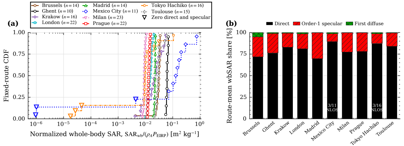
FIGURE 5. Normalized whole-body SAR on the ten fixed routes. (a) Empirical CDFs include all 163 route points. Hollow triangles mark the six points with zero direct and zero order-1 specular transfer. (b) Route-mean component shares of whole-body SAR. The routes are fixed case studies, not city or population samples.
