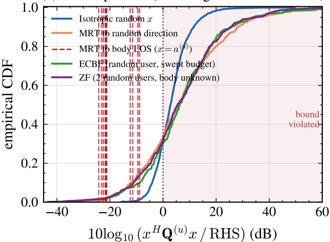
(a) Plaza specular (LOS + ground + 2 facades)
