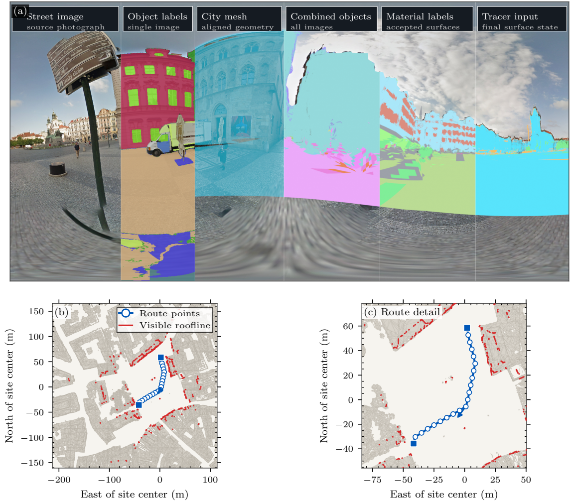
FIGURE 1. Study configuration at Prague Old Town Square. Panel (a) follows a 360-degree street image through object segmentation, projection onto the city mesh, and conversion to the material map used by the tracer. Panel (b) shows the 22 route points and the visible roofline on a plan view of the city. Panel (c) enlarges the route. The arrow gives the phantom's direction along the walk.
