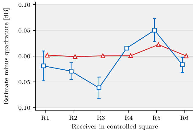
(b) Error against surface quadrature
