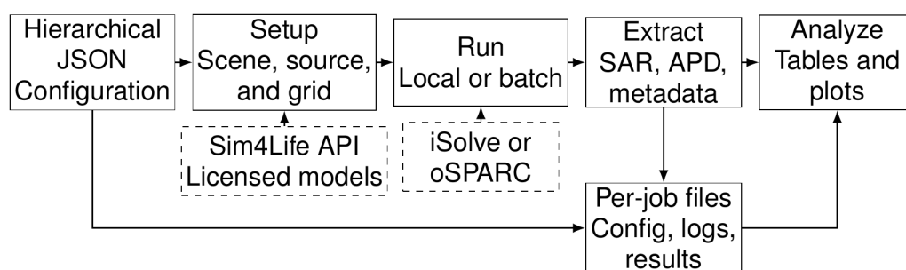
Figure 1: GOLIAT flowchart. The top row shows a study from hierarchical configuration to analysis. Dashed boxes mark licensed models and external execution services. Each simulation has a separate configuration, log, and result record.
