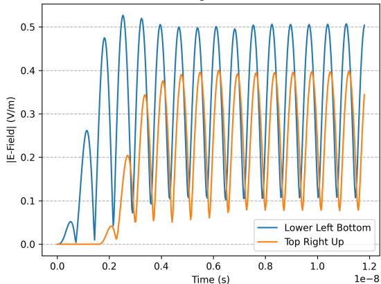
Point Sensor E-Field Magnitude vs. Time (700 MHz)
