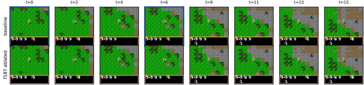
Supplementary Figure S7: f_{187} is a code-only lesion: the suppressed state is carried by the frame, not the code . Paired decoded imagination for a collect_wood moment, baseline (top) vs wood-feature ( f_{187} ) ablation (bottom); the orange box marks the HUD inventory/vitals strip (rows y \geq 49 ), a blue frame marks a step where the wood detector code is sampled. Under ablation the wood code is never sampled (blue frames vanish), yet the HUD inventory strip still renders the wood the agent holds: its mean absolute pixel difference from baseline is only 2.2/255 , versus 20.4/255 ( \approx 9.4\times ) in the world view above. Because the convolutional encoder re-reads the inventory from each frame, the downstream wooden-item codes can fire from this frame-carried state that the suppressed code never gated—the mechanism behind the powered behavioural null in Fig. S6.
