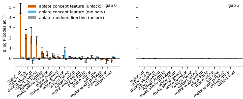
Fig. 4 Single-step causal ablation. Change in log-likelihood of the observed codes at the target step when the concept’s SAE direction is projected out of the block-1 residual stream, at the target step itself (left) or three steps earlier (right); n=80 moments per bar (26–29 for two concepts), error bars are bootstrap 95% CIs. Red: matched direction at unlock moments. Light blue: matched direction at ordinary moments. Grey: random direction at unlock moments. Effects are direction- and moment-selective at gap 0 and vanish entirely at gap 3.
