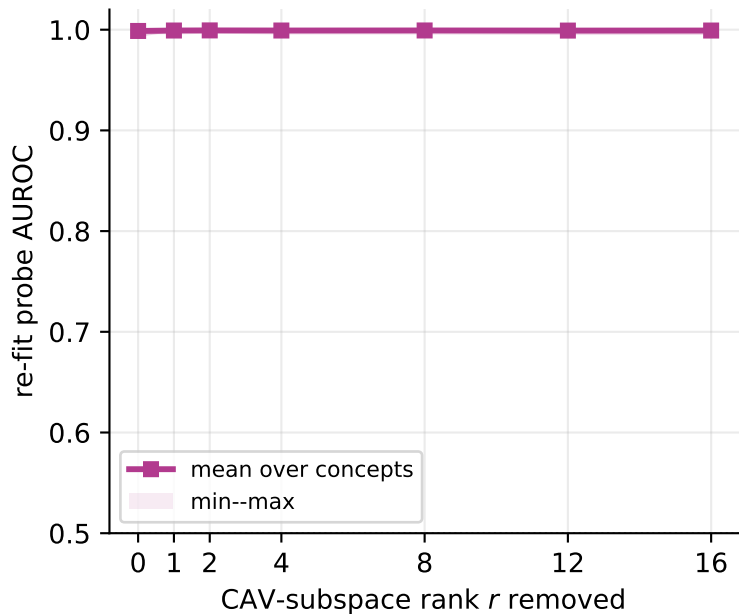
(B) Decodability survives removal
