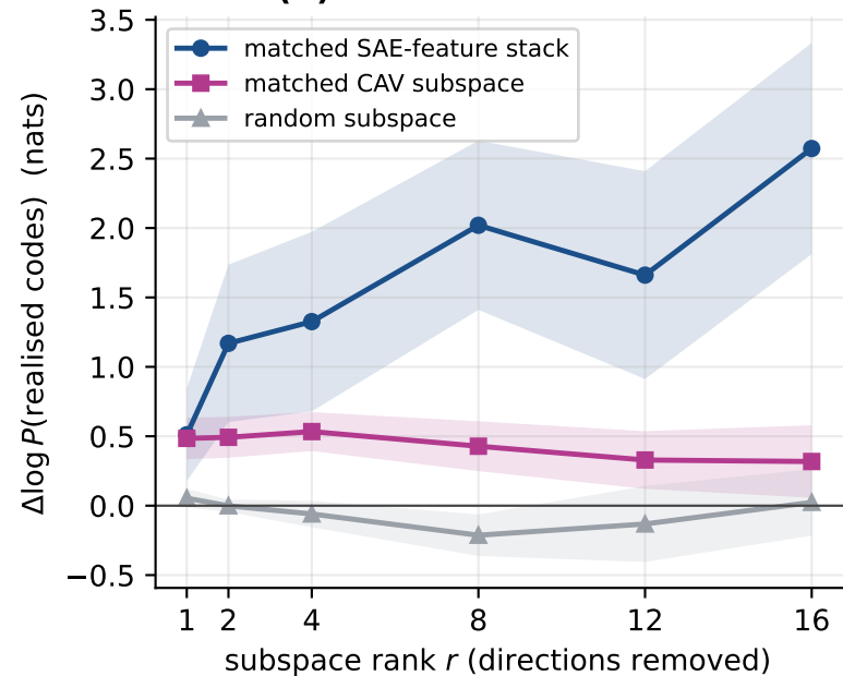
(A) Causal effect vs rank
