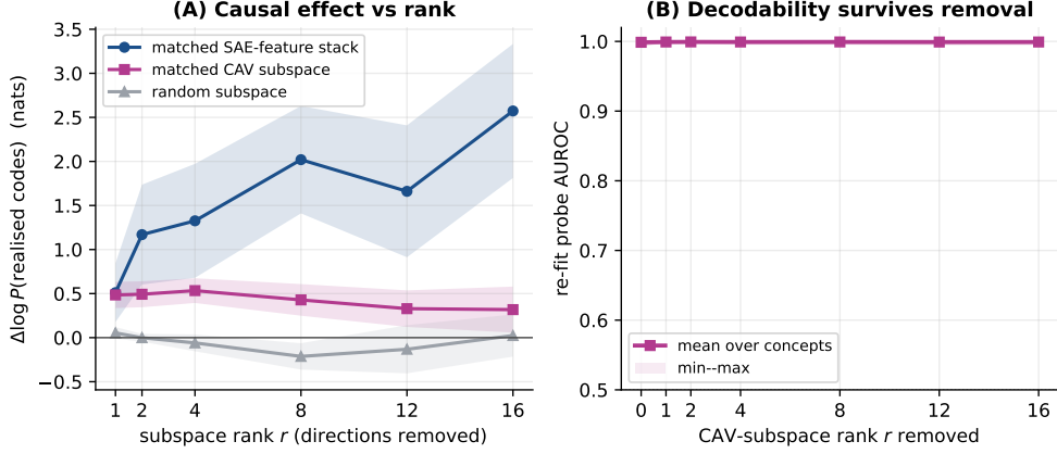
Fig. 7 Multi-direction (INLP-style) ablation, single-step, unlock moments. (A) mean \Delta \log P of the realised codes (over eight dominant concepts; band = \pm SEM) when a rank- r orthonormal subspace is projected out of the block-1 residual stream: the matched SAE-feature stack climbs with rank, the matched CAV subspace saturates \sim 0.5 nat ( \approx 8\times smaller at r=16 ), the random subspace is inert. (B) AUROC of a probe re-fit after projecting out the rank- r CAV subspace: decodability survives ( \approx 0.999 ) up to r=16 , evidencing massive redundancy. Together: probe-decodable concept information is redundant and is not what the model writes through; the dictionary basis is.
