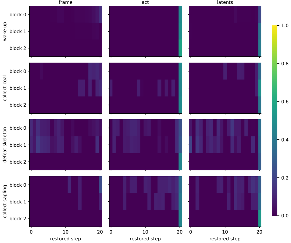
Fig. 7 Causal tracing. Mean restoration of unlock-code prediction when clean activations are patched into a corrupted run, per (block \times timestep) cell, for frame, action and latent token positions (columns) and four concepts (rows). Restoration concentrates entirely at the final (unlock) timestep, dominated by the action and latent tokens; patching any historical cell restores essentially nothing.
