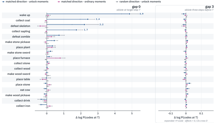
Fig. 5 Single-step causal ablation. Change in log-likelihood of the observed codes at the target step when the concept’s SAE direction is projected out of the block-1 residual stream, at the target step itself ( gap 0 , left) or three steps earlier ( gap 3 , right); markers show the mean change, whiskers are bootstrap 95% CIs, n=80 moments per condition (26–29 for two concepts). Blue: matched direction at unlock moments. Magenta: matched direction at ordinary moments. Grey: random direction at unlock moments. The gap-3 panel is drawn in a framed inset on an expanded ( \times 9 ) horizontal scale so that the near-zero effects and their confidence intervals are visible; every interval crosses zero. Effects are direction- and moment-selective at gap 0 and vanish entirely at gap 3.
