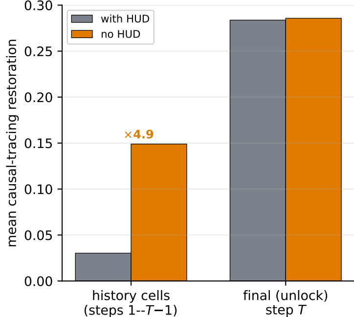
(B) De-Markovianisation of next-code prediction
