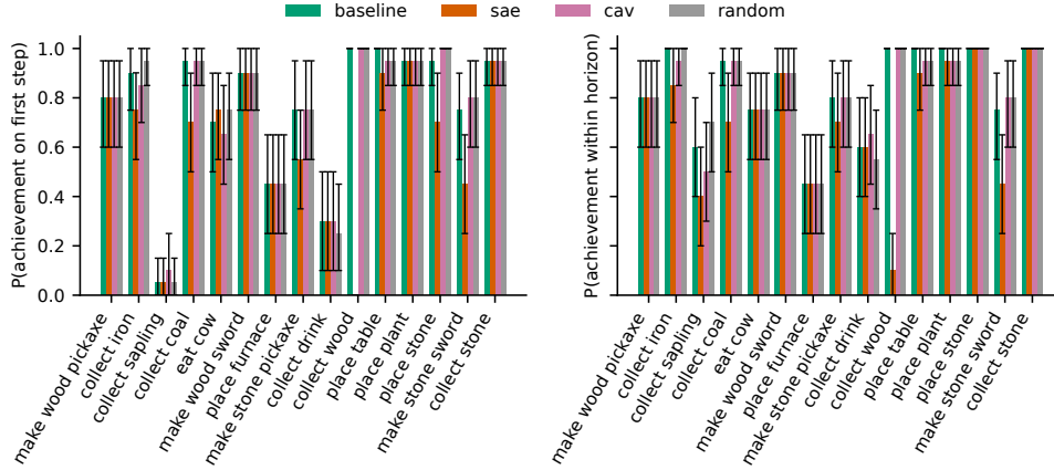
Fig. 5 Concept-direction ablation inside 12-step imagination, for the 15 of 18 concepts whose baseline within-horizon detector probability is at least 0.4. Bars: probability that the concept’s detector code is sampled at the first imagined step (left) and within the horizon (right) under no intervention (baseline), SAE-direction ablation, CAV-direction ablation and random-direction ablation; bootstrap 95% CIs, n=20 rollouts per bar.
