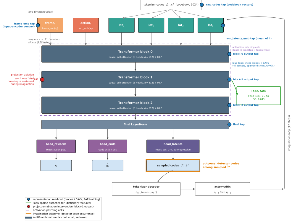
Fig. 1 Overview of the audit. Grey-blue components reproduce the \Delta -IRIS world model of Micheli et al. [6] (redrawn from the reference implementation): per timestep, a frame embedding, an action embedding and four tokenizer codes enter a 3-block causal transformer, and three heads predict reward, termination and the next four codes autoregressively. Coloured elements are our contribution—the audit instrumentation: blue taps mark the seven representation read-out points used for linear probes and CAVs (Section 6), including the frame_emb input-encoder control behind the HUD-shortcut analysis; green, the TopK sparse autoencoder trained on the block-1 output (Section 7); red, the projection-ablation intervention point (Equation 2, Sections 8.1–8.2); purple dashes, the activation-patching cell grid (Section 8.3); orange, the imagination-loop outcome (detector-code occurrence among sampled codes). A detailed view of the heads’ read positions is given in Appendix B.
