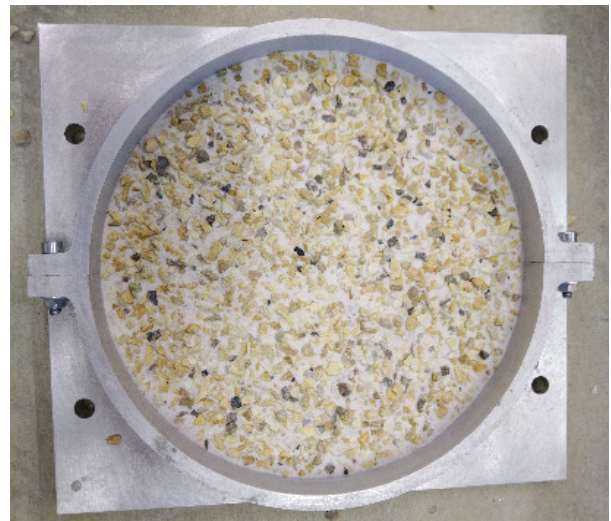
(b) Put a single layer of sands on the aggregates
