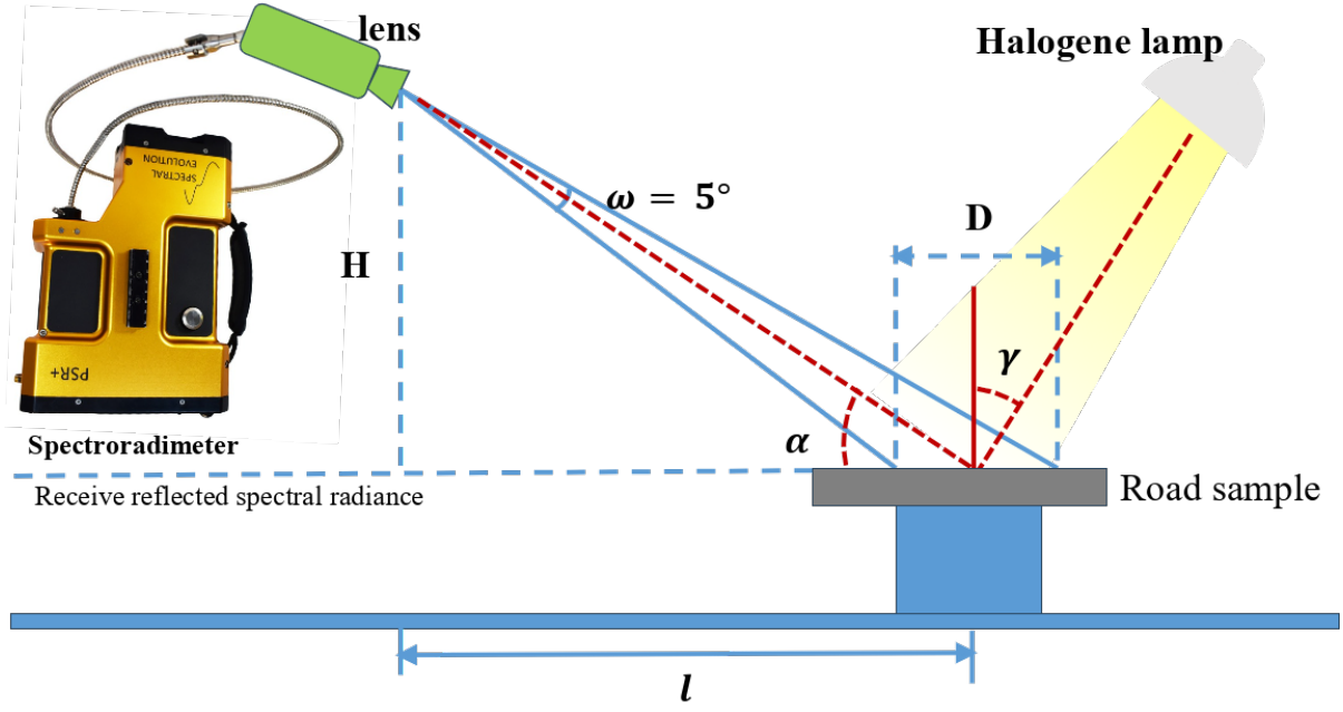
Figure 5.9: Gonio-spectroradiometer (Cerema)
