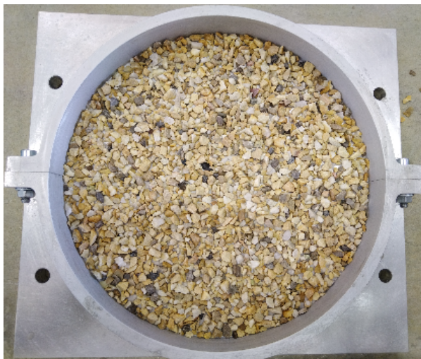
(a) Put a single layer of aggregates on the mould
