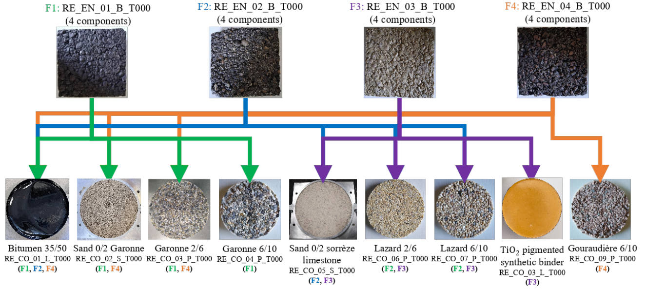
Figure 5.1: 4 formulations of roads and their components
