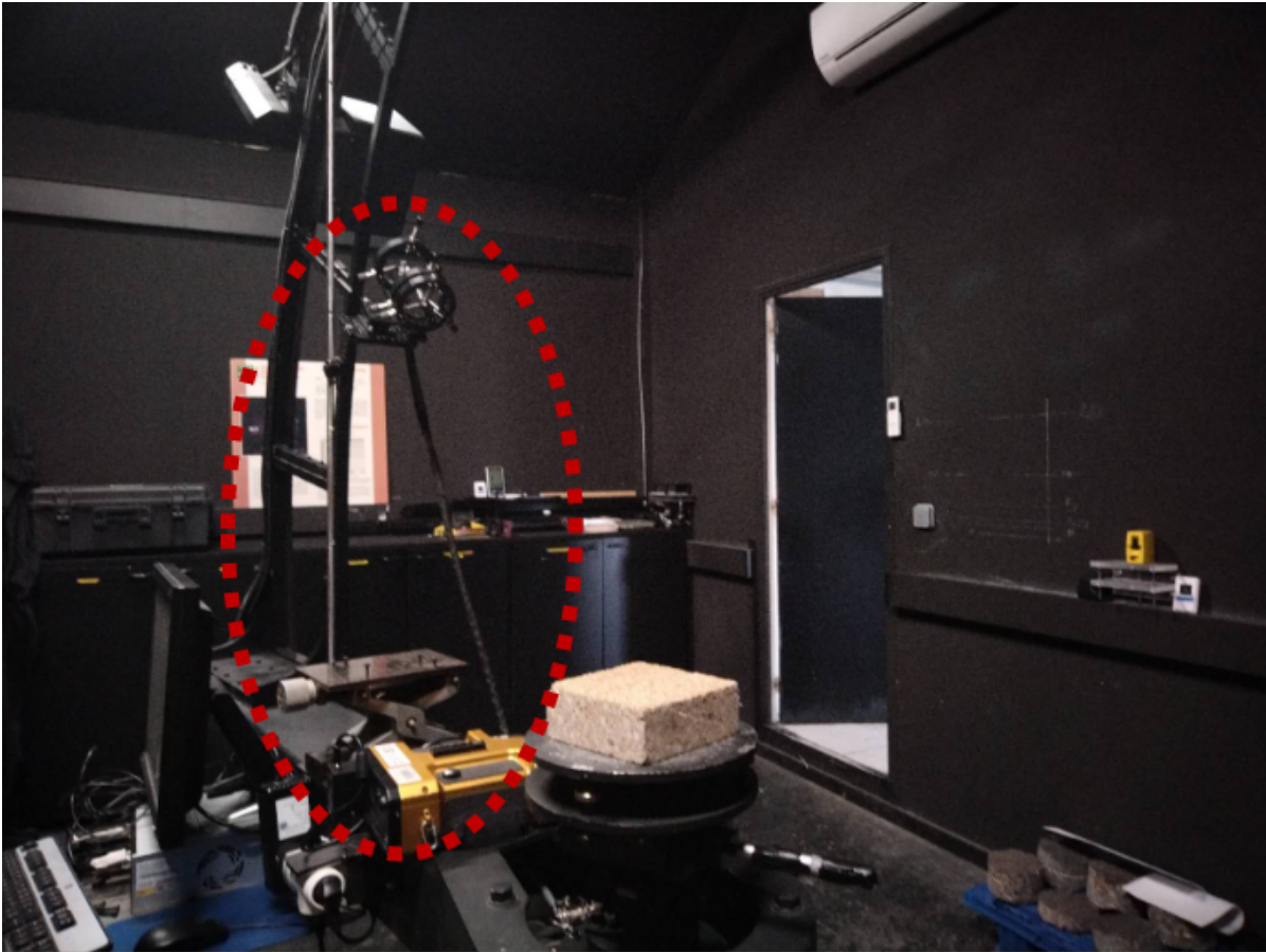
Figure 5.8: Gonio-spectroradiometer (Cerema)
