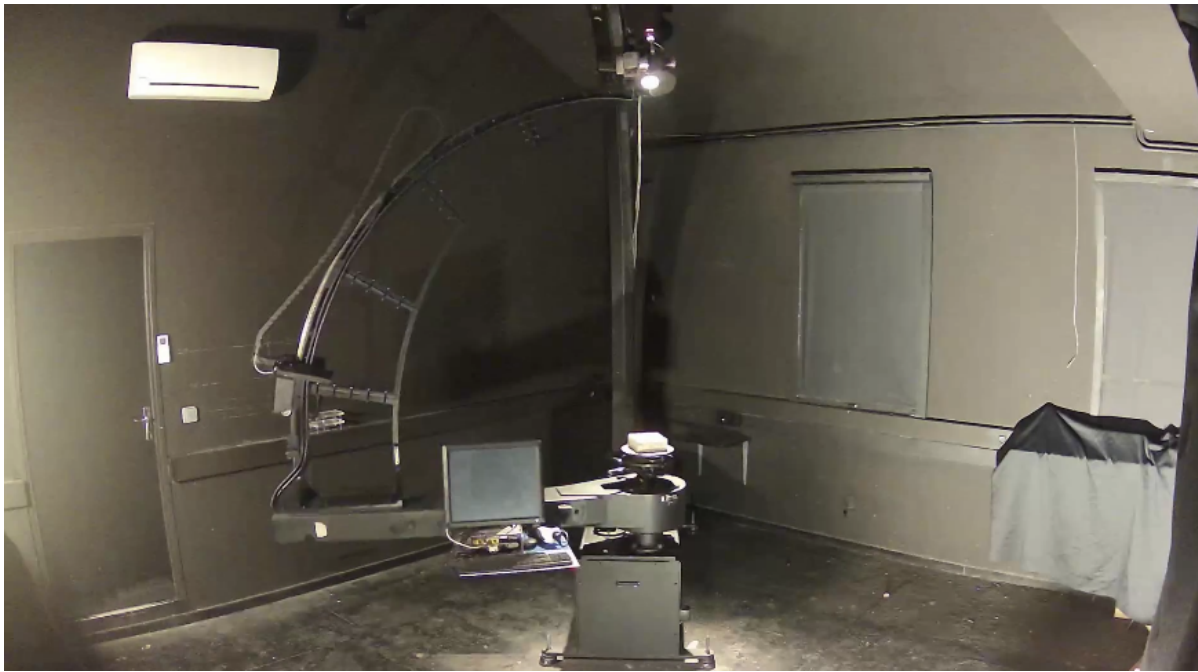
Figure 5.7: Gonioreflectometer (Cerema)
