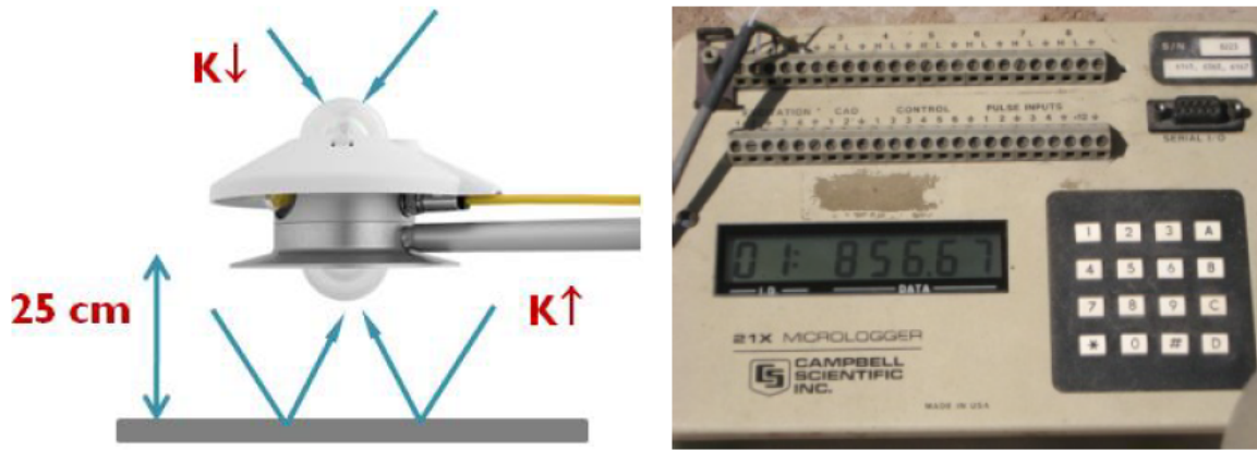
Figure 4.17: Two coupled-pyranometers (left) and a multi channel data logger
