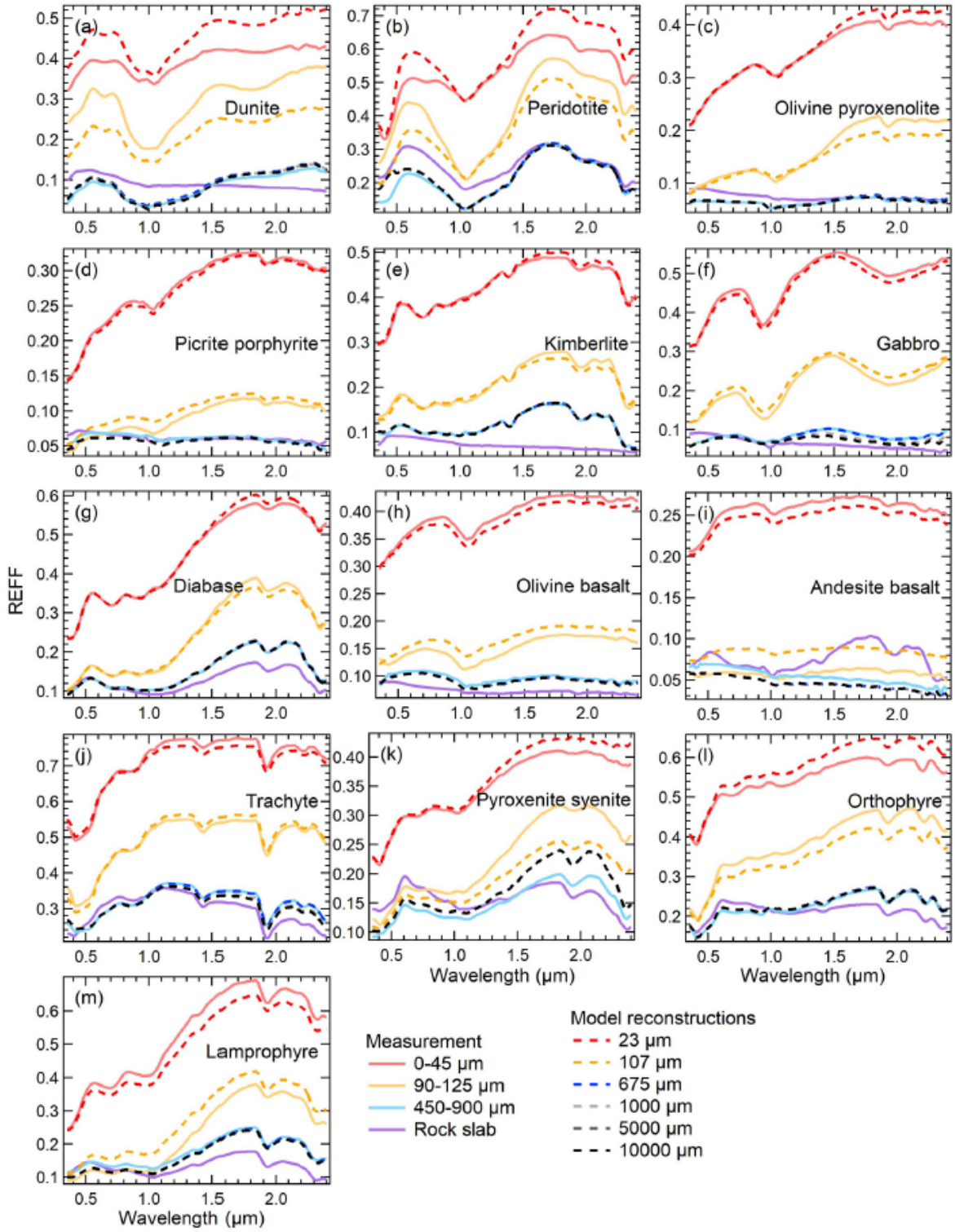
Figure 4.11: Igneous rocks: Hapke's SHOE model fitting to measured RE_{\text{eff}}
