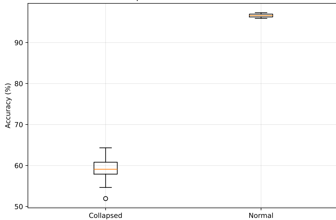
Collapsed vs Normal Distribution
