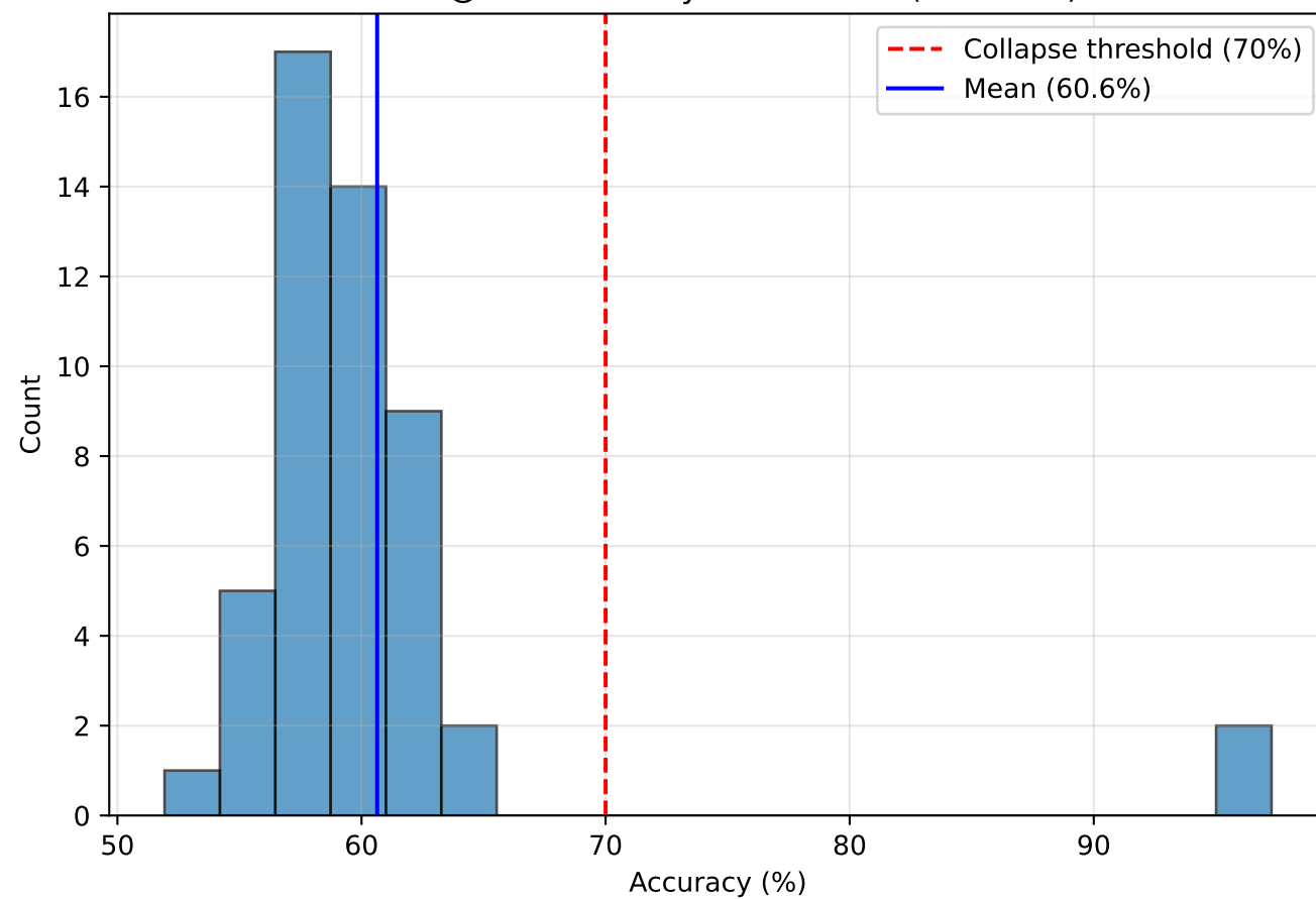
Collapsed vs Normal Distribution
