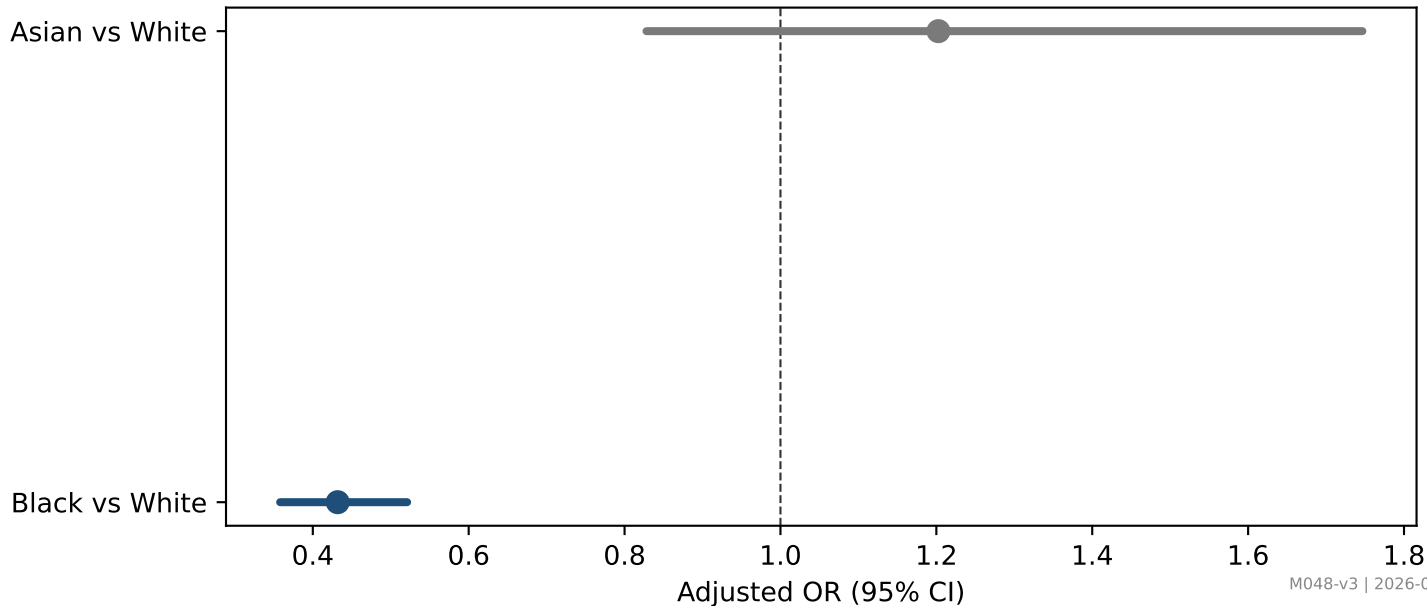
Figure 6 — Model F race effects (full adjustment)
