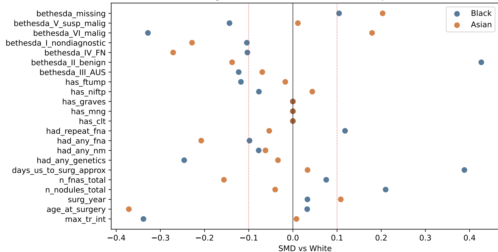
Figure 10 — Covariate balance (Love plot)
