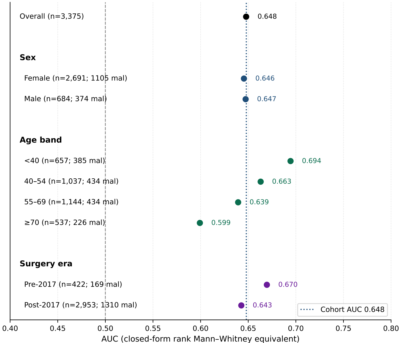
Figure 5. Subgroup forest plot — AUC by demographic stratum Discrimination is preserved (modest) across sex, age, and era
