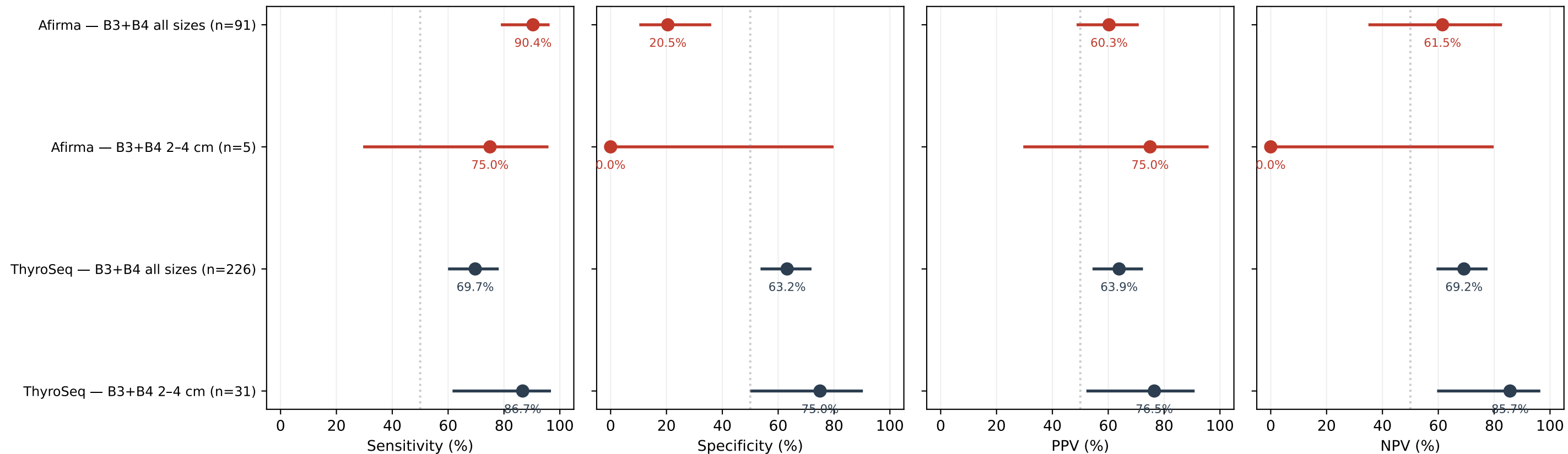
Figure 2. Diagnostic performance of Afirma and ThyroSeq in surgical Bethesda III/IV cohort (actual platform-reported call; Wilson 95% CIs; NIFTP coded as benign)
