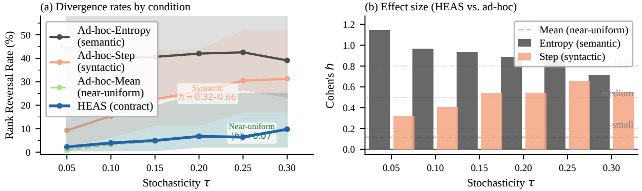
Figure 2: Contract divergence prevention across \tau \in [0.05, 0.30] ( n = 25/\text{condition/level} ). Left : rank reversal rate (%) with 95% Wilson CI. Three regimes: semantic ( h = 0.72-1.14 , Entropy); syntactic ( h = 0.32-0.66 , Step); near-uniform ( |h| < 0.07 , Mean). Right : Cohen’s h — contract benefit scales with aggregation heterogeneity, not noise level.
