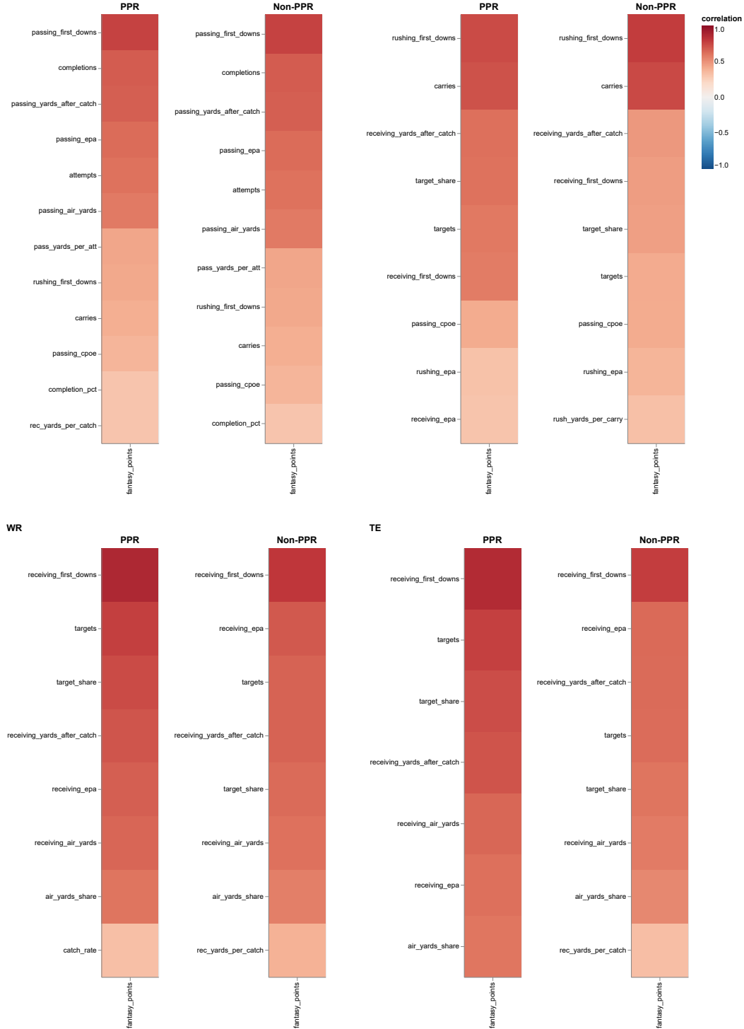
Stats Correlated with Fantasy Points by Position ( |r| \geq 0.3 )
