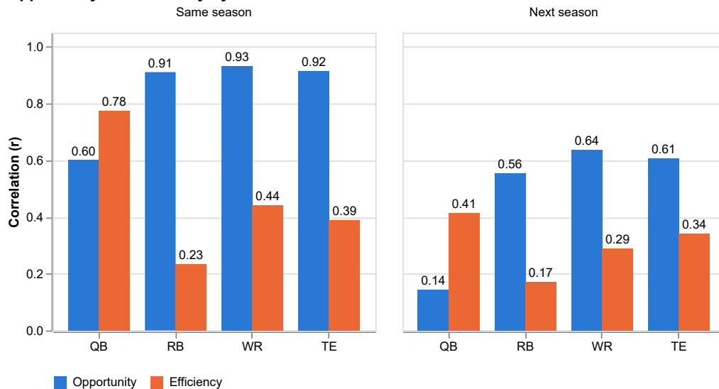
Opportunity vs. Efficiency by Position
