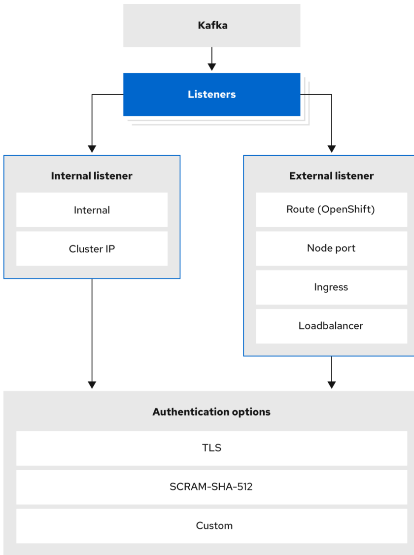
Figure 3. Kafka listener authentication options
