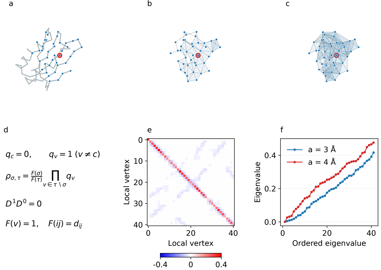
Figure 2: Local spectral descriptor construction. (a) The fixed 13 \text{ \AA} support around residue 43 of chain A in 1ULR contains 41 C_\alpha vertices; red identifies the center. (b,c) Alpha complexes at ball radii 3 and 4 \text{ \AA} retain those vertices while adding edges and triangles. (d) Compatible center-zero restrictions define a cochain complex. The figure's d_{ij} = \|x_i - x_j\|/(1 \text{ \AA}) is the dimensionless distance denoted r_{ij} in the text. (e) The degree-zero center-zero Laplacian at a = 4 \text{ \AA} , with local-vertex indices on both axes. (f) Ordered eigenvalues at the two scales. These are geometric operators and spectra, prior to fitting a B-factor model.
