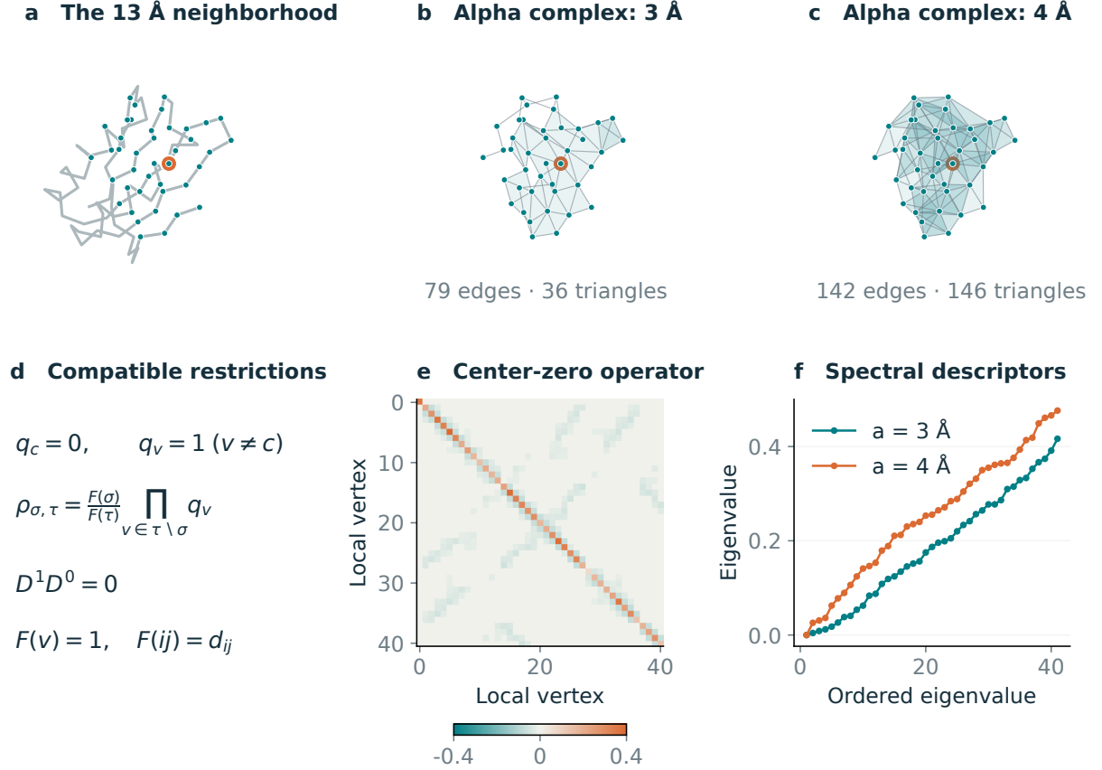
Figure 2: From a residue neighborhood to local spectra. (a) The fixed 13 Å support around residue 43 of chain A in 1ULR contains 41 C_\alpha vertices; orange identifies the center. (b,c) Alpha complexes at ball radii 3 and 4 Å retain those vertices while adding edges and triangles. (d) Compatible center-zero restrictions define a cochain complex. The figure’s d_{ij} = \|x_i - x_j\|/(1 \text{ Å}) is the dimensionless distance denoted r_{ij} in the text. (e) The degree-zero center-zero Laplacian at a = 4 \text{ Å} , with local-vertex indices on both axes. (f) Ordered eigenvalues at the two scales. These are geometric operators and spectra, prior to fitting a B-factor model.
