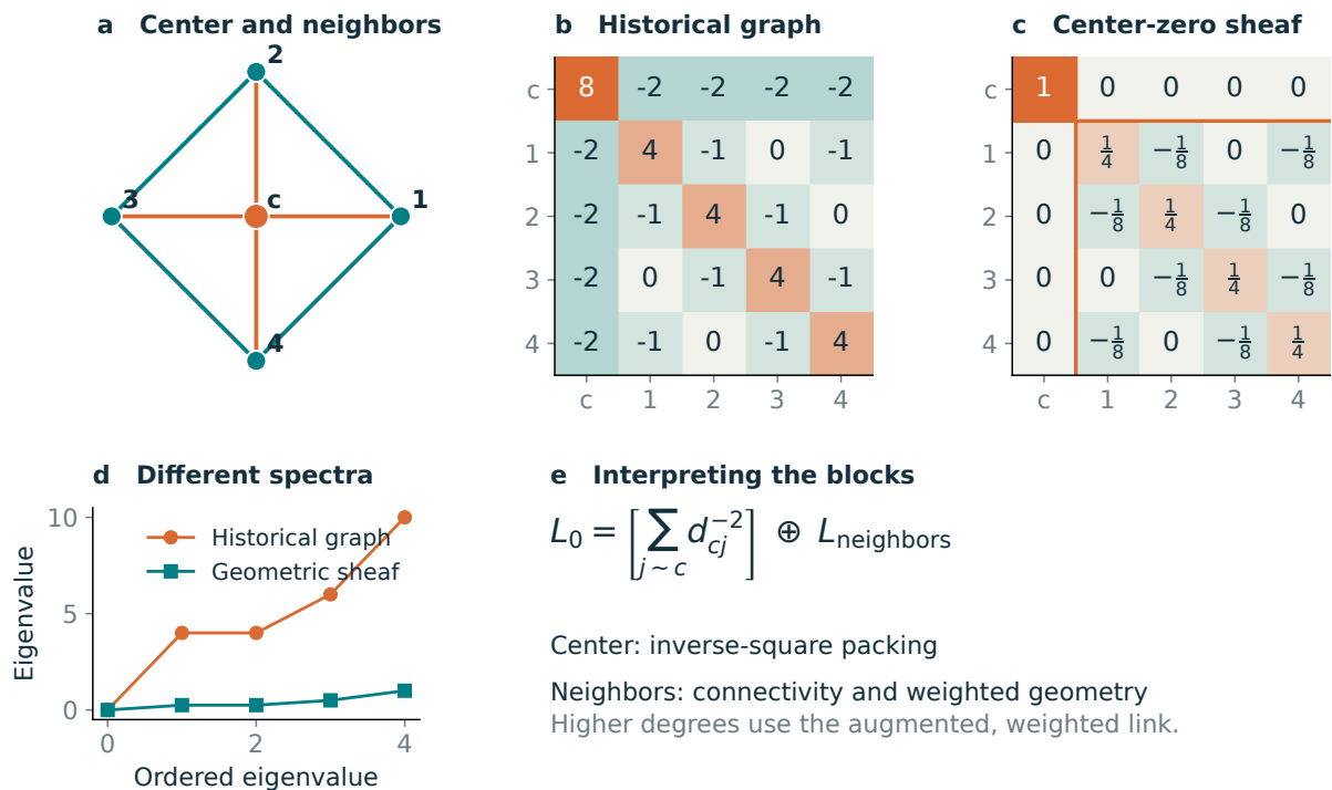
Figure 3: Two center-label constructions on an illustrative five-point geometry. (a) The center is at (0, 0, 0) and four neighbors at (\pm 2, 0, 0) and (0, \pm 2, 0) Å. The native contact radius and the alpha radius are both 3 Å in this example. (b,c) The native graph Laplacian couples the center to every neighbor; the geometric center-zero degree-zero sheaf Laplacian separates a center scalar from the deletion graph. (d) Their spectra are \{0, 4, 4, 6, 10\} and \{0, 0.25, 0.25, 0.5, 1\} , respectively. (e) The center scalar is an inverse-square packing sum, with d_{cj} = \|x_c - x_j\|/(1 \text{ Å}) . The augmented weighted link gives the higher-degree generalization. Matrix colors describe algebraic entries, not mechanical components.
