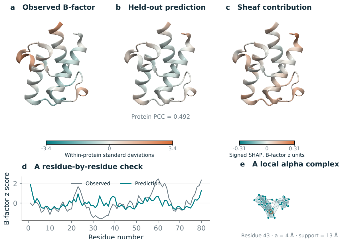
Figure 6: The predetermined companion protein 1X3O. (a,b) Observed within-protein normalized B-factor and the sequence-cluster-held-out graph-plus-center-zero prediction, mapped to the same residue coordinates and shown with a common color scale. (c) The signed sum of TreeSHAP contributions from the 24 center-zero spectral features, in B-factor z-score units. This subtotal excludes graph-feature contributions and the training-background expectation; teal is negative and orange positive. (d) Observed and predicted residue profiles provide a direct check alongside the structural views. (e) The local alpha complex at ball radius 4 Å within the fixed 13 Å support of the labeled residue. The protein, model protocol, and feature grouping were specified before inspecting prediction outcomes.
