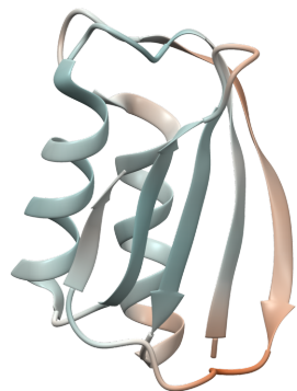
a Observed B-factor
