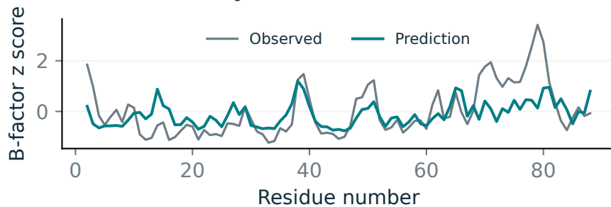
d A residue-by-residue check
