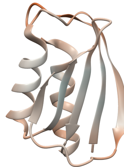
Sheaf contribution
