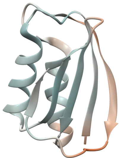
Observed B-factor
