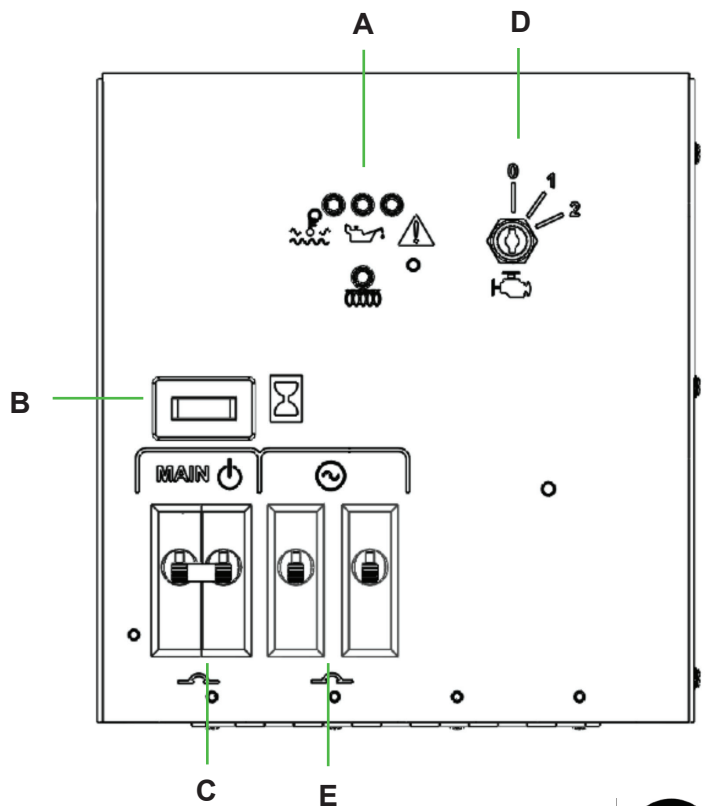
Figure 3-1 Main Control panel
