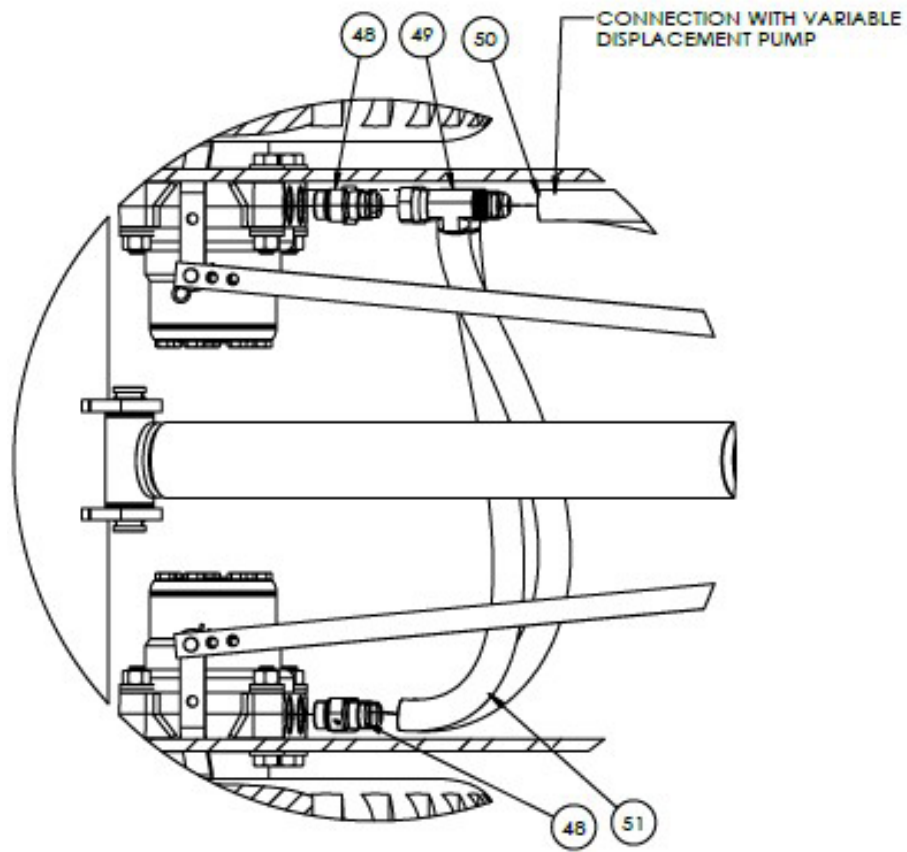
DETAIL D SCALE 1 : 4
