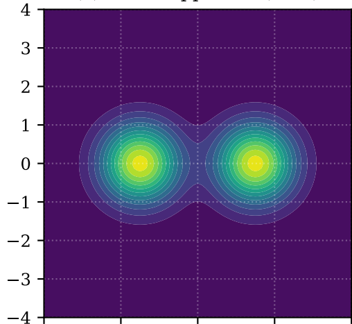
(a) Initial Approach ( t = 0 )
