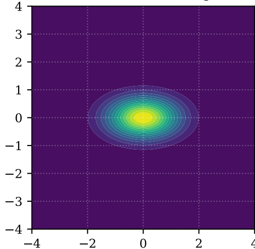
(c) 90^\circ Transverse Scattering ( t = 24\tau_0 )
