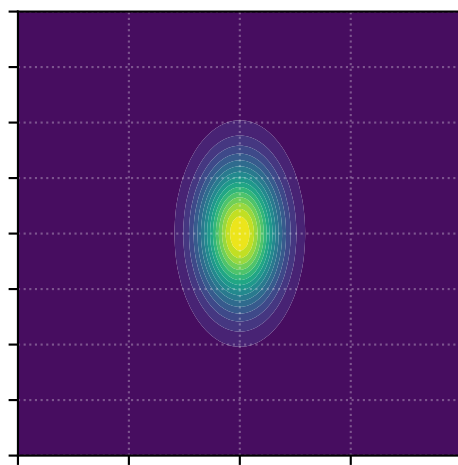
(b) Core Compression ( t = 12\tau_0 )
