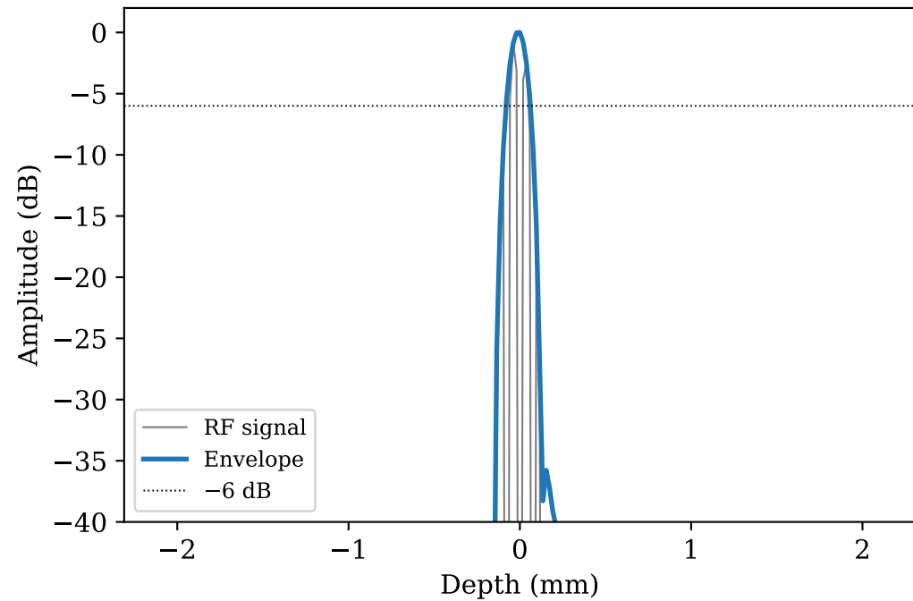
Axial PSF Envelope
