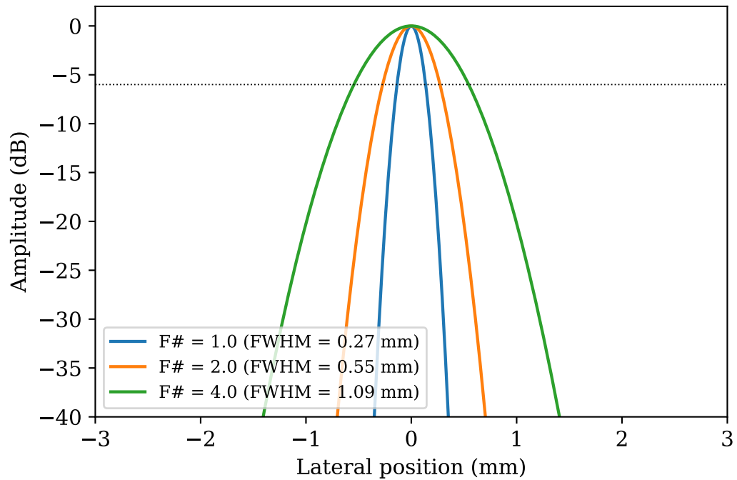
Lateral PSF — f_0 = 5 MHz
