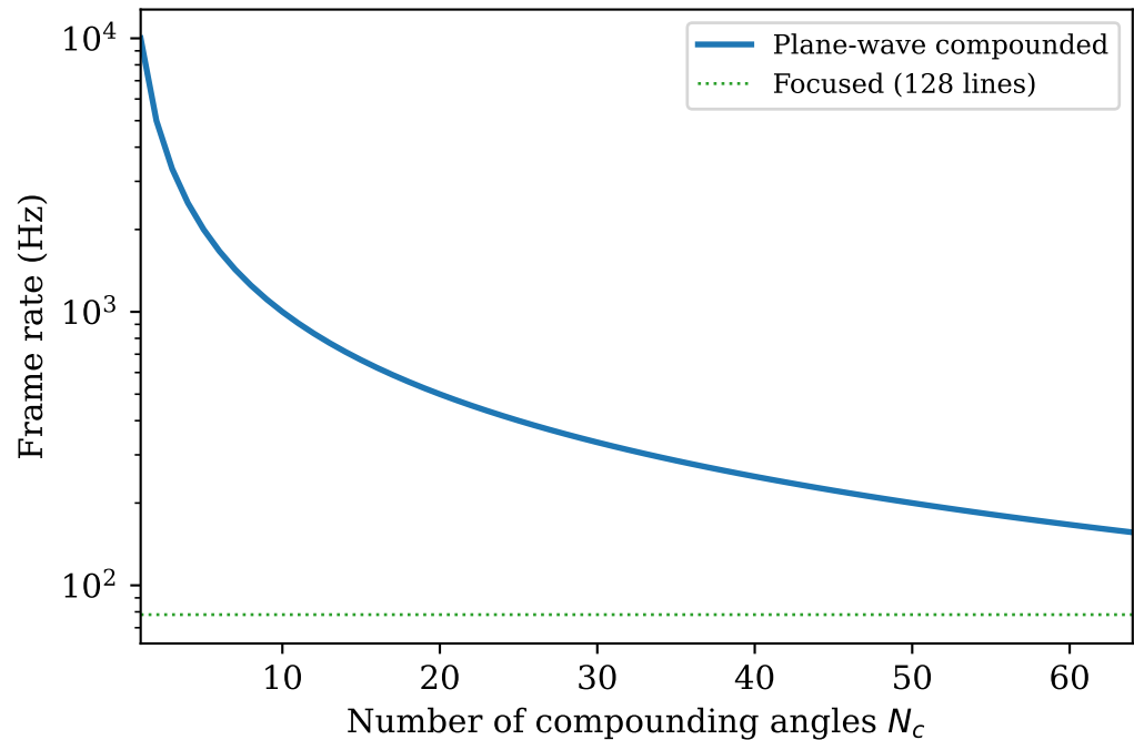
Frame Rate vs Compounding Angles (PRF = 10 kHz)
