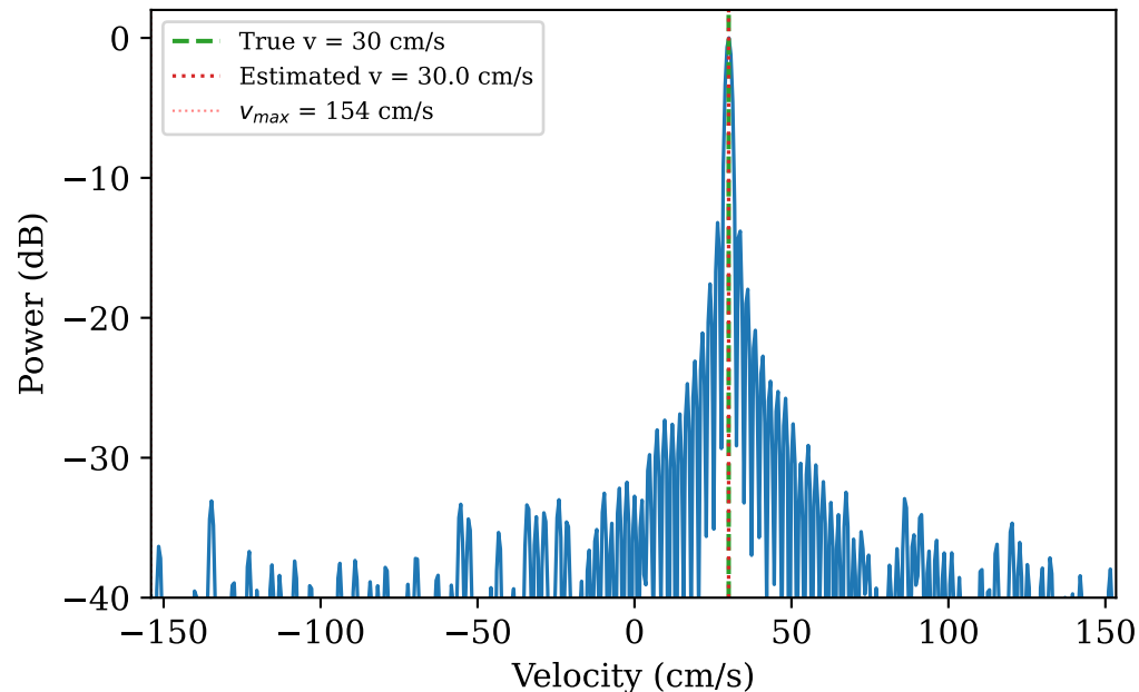
Contrast-Agent Doppler Spectrum — f_0 = 5\ \text{MHz} , \alpha = 60.0^\circ RP amplitude: A_{bubble} = 0.183 (pykwavers.solve_rayleigh_plesset)
