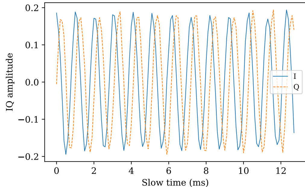
Slow-time IQ — contrast agent R_0 = 1.5\ \mu\text{m} , P_a = 100\ \text{kPa}
