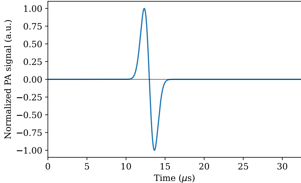
PA Waveform at Surface Sensor
