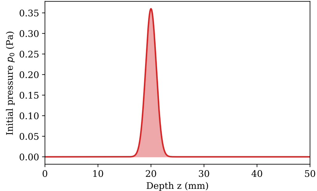
Photoacoustic Initial Pressure (Eq. 5.18) \Gamma = 0.18, \mu_a = 100.0 \text{ m}^{-1}, \Phi = 0.02 \text{ J/m}^2
