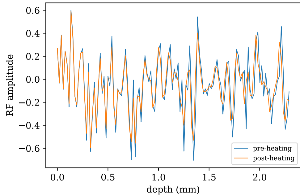
(a) RF echo shift from heating
