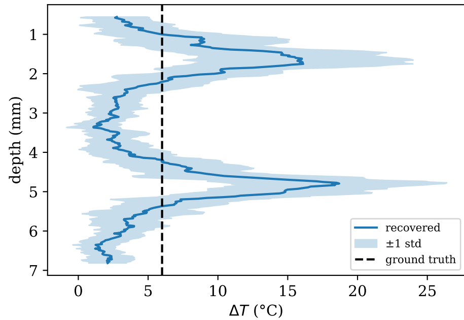
(c) Reconstructed \Delta T ( k_T = -9.99e - 04/^{\circ}\text{C} )
