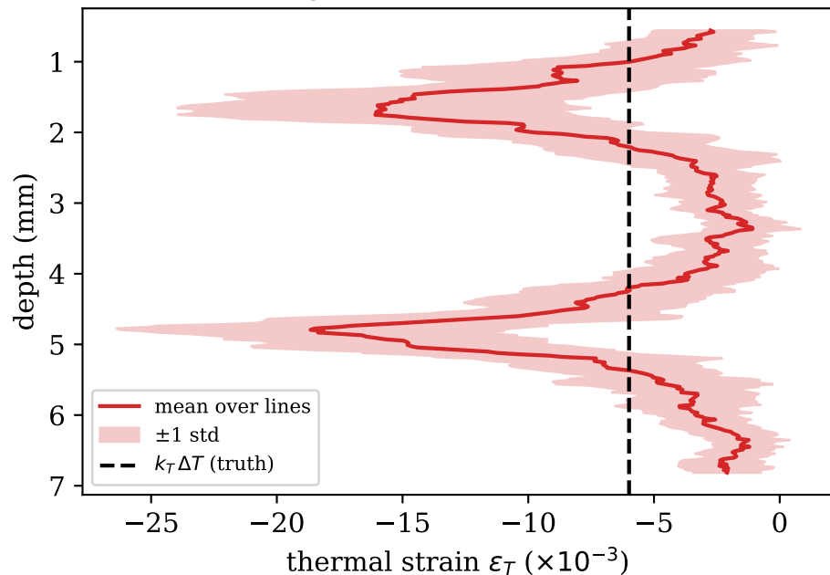
(b) Negative strain (water-based)
