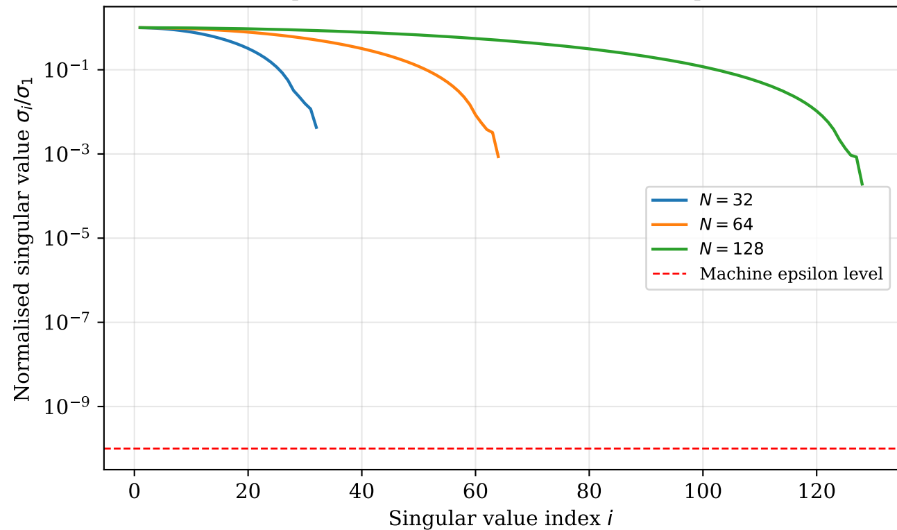
SVD spectrum of 1D Helmholtz forward operator
