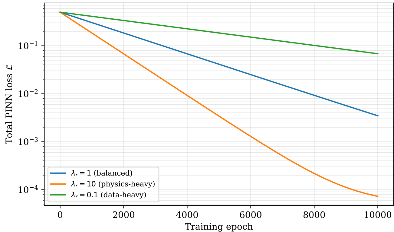
PINN convergence illustration: \mathcal{L} = \mathcal{L}_{\text{data}} + \lambda_r \mathcal{L}_{\text{PDE}}
