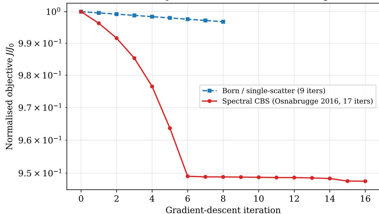
CBS FWI convergence: Born vs spectral CBS 10×10×1 phantom, 200 kHz, 8-element ring
