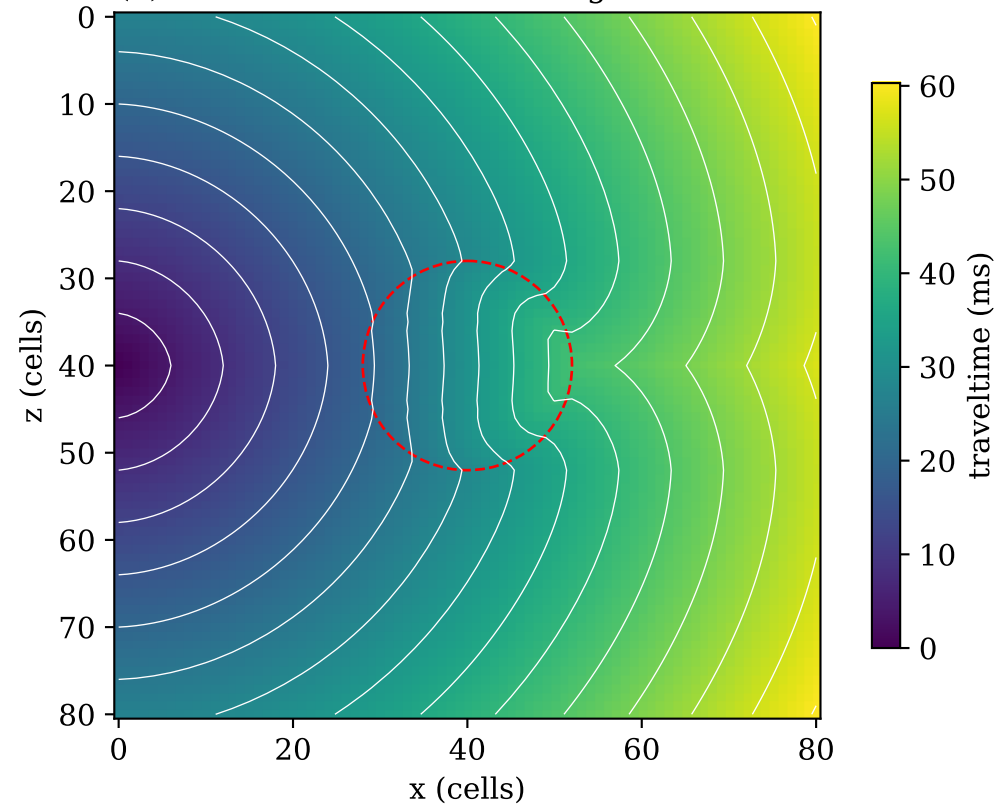
(a) Eikonal traveltimes through a slow lens
