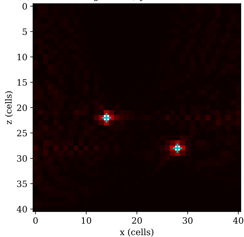
(b) Kirchhoff migration (cyan + = true scatterers)
