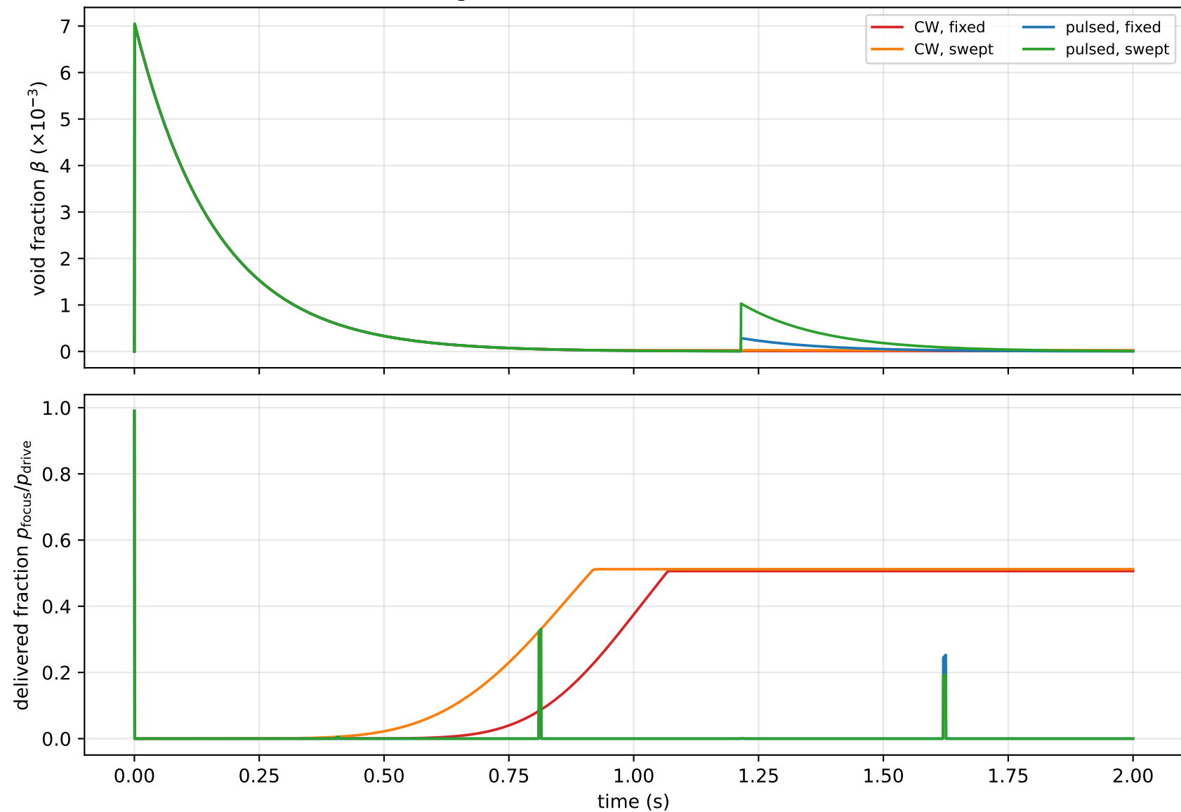
Cavitation-shielding control: void fraction and delivered transmission
