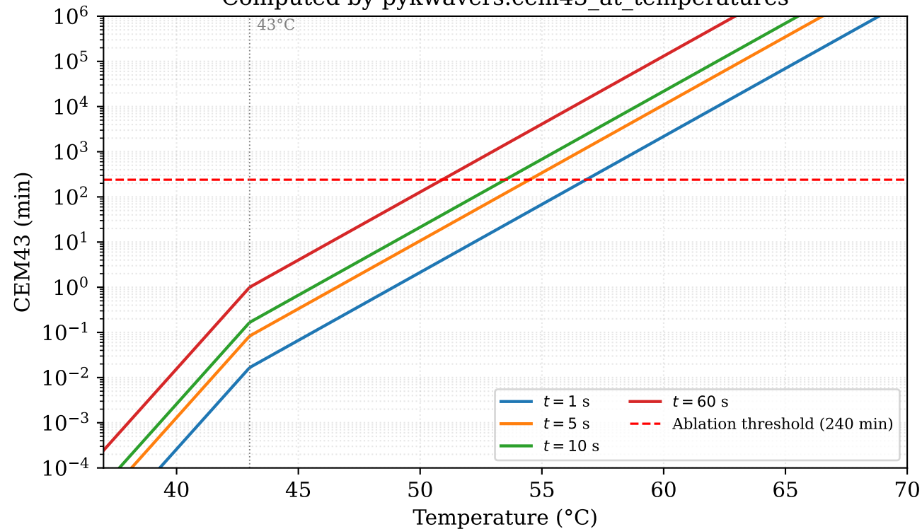
Thermal Dose Accumulation (Eq. 6.7, Sapareto & Dewey 1984) Computed by pykwavers.cem43_at_temperatures
