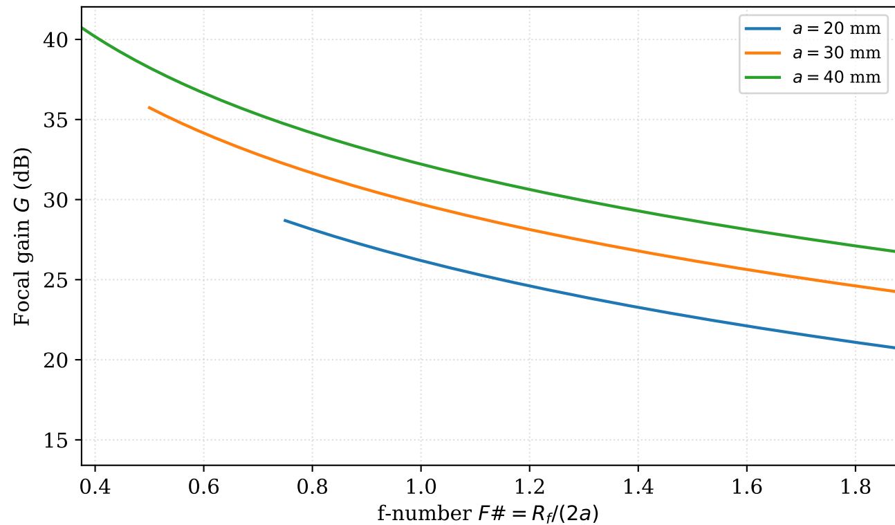
HIFU Focal Gain (Eq. 6.2) — f_0 = 1 MHz
