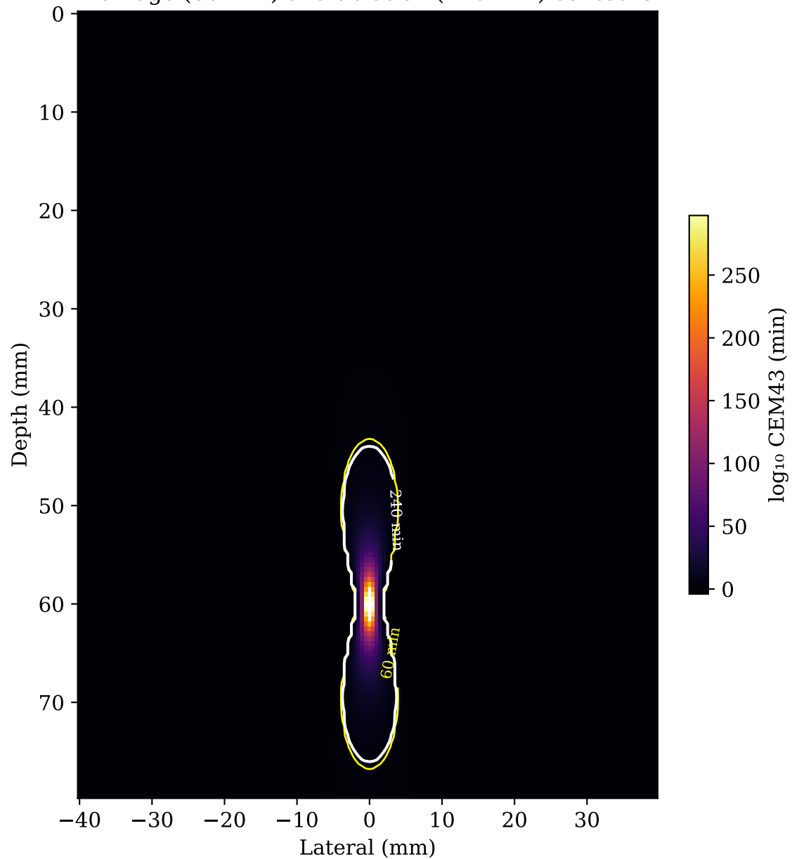
CEM43 Thermal Dose [ \log_{10} min] Damage (60 min) and ablation (240 min) contours
