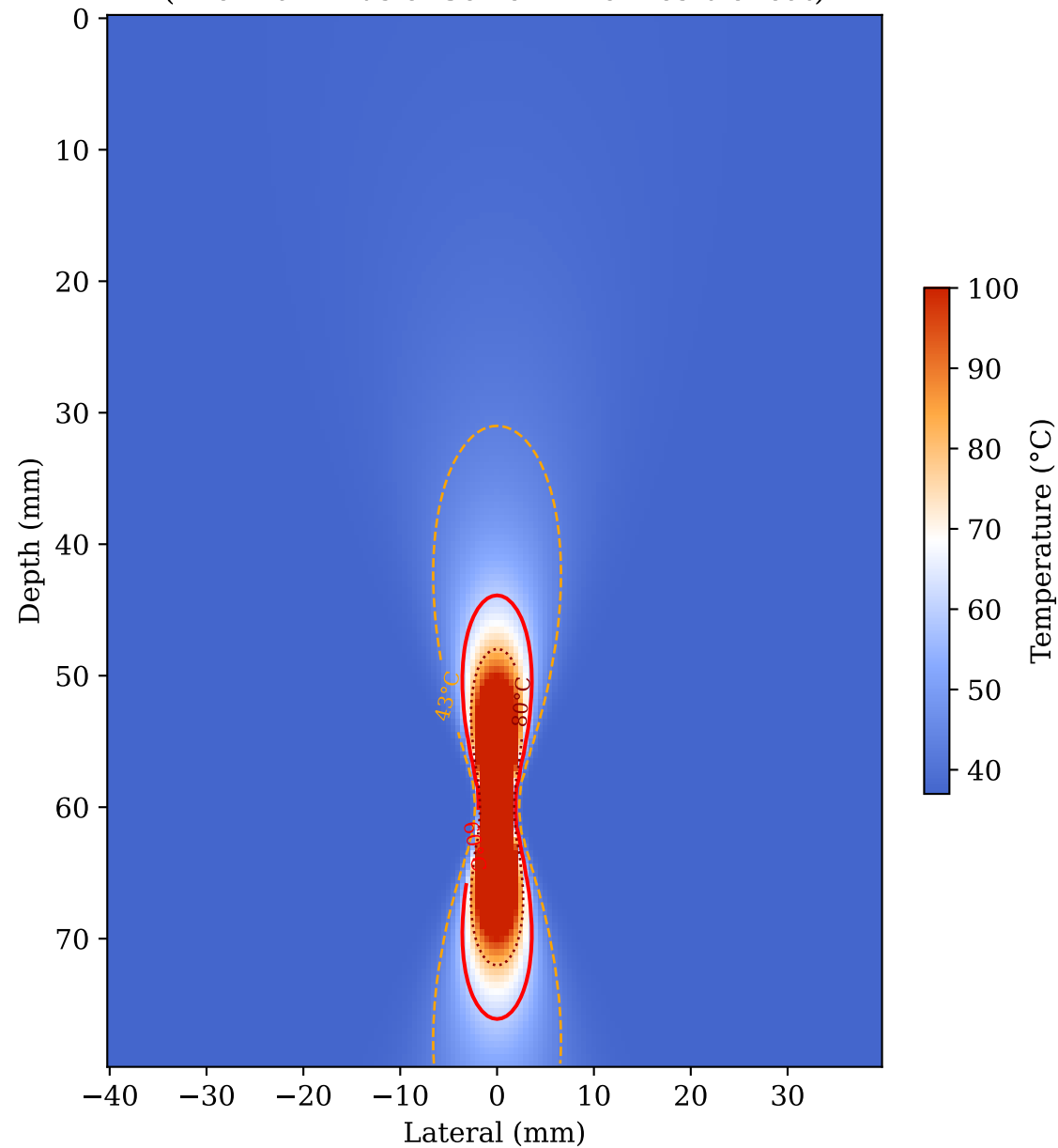
Temperature — HIFU, 1 s sonication (ThermalDiffusionSolver + Pennes bioheat)
