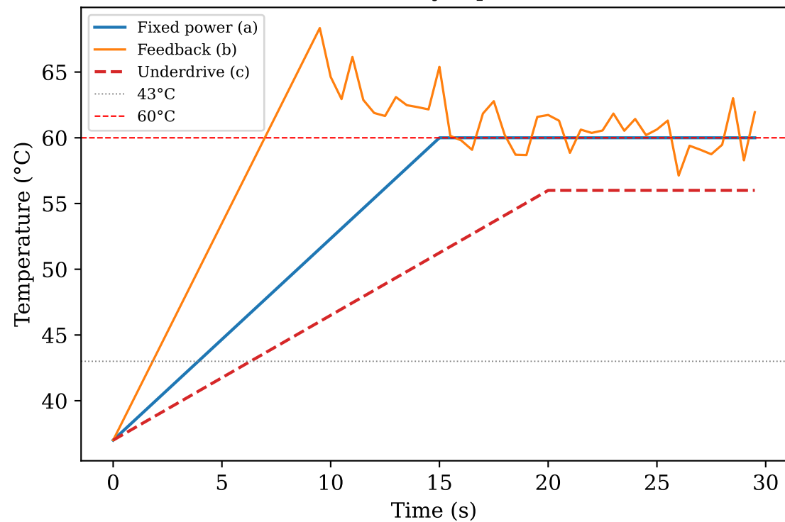
Controlled Focal Temperature — Clinical HIFU (MR thermometry representation)
