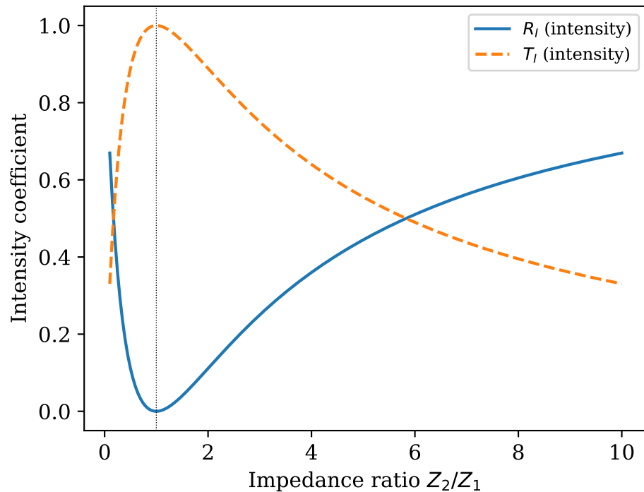
Intensity reflection/transmission
