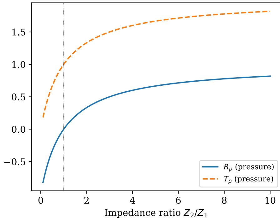
Pressure reflection/transmission
